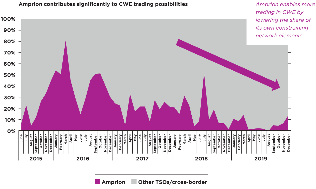
Figure: Decreasing share of Amprion's market-constraining internal network elements, i.e. relative frequency of active critical branches per hour from 06/2015-12/2019 Please note that only internal network elements are shown
