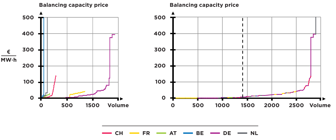
Figure 23: Exemplary structure of single and common merit order lists on 16 of November 2019
