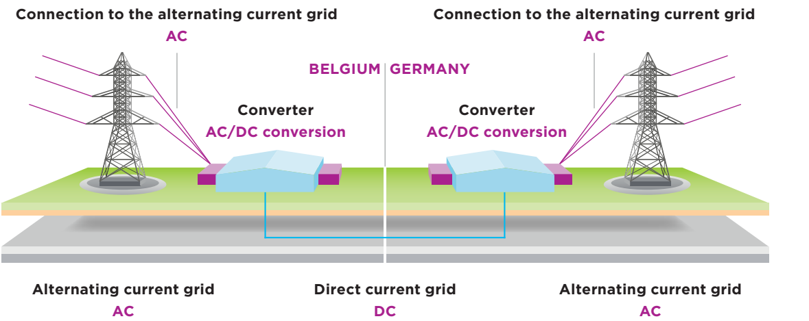
Figure 24: DC technology for ALEGrO
